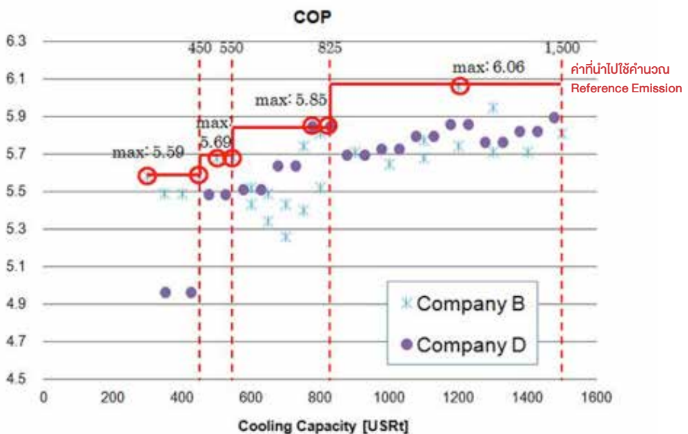
Figure 1: COP values of inverter type centrifugal chiller marketed in Thailand
